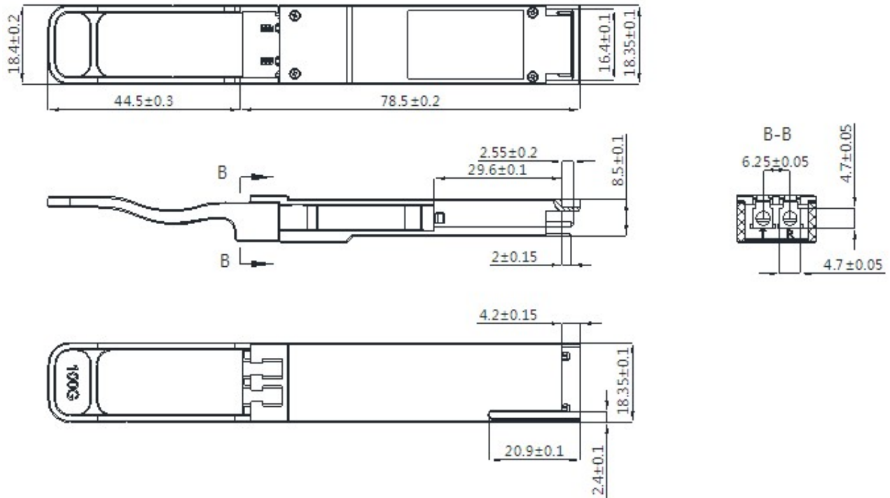
Figure 5. Outline Drawing
