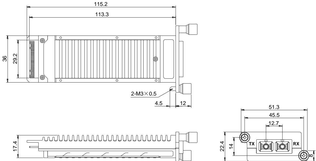
Figure 4. Outline Drawing
