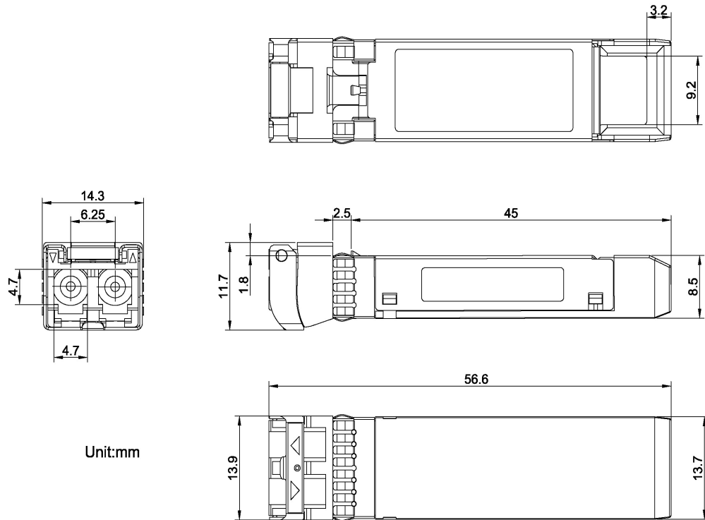
Figure 4. Outline Drawing
