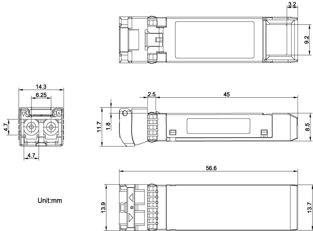
Figure 4. Outline Drawing
