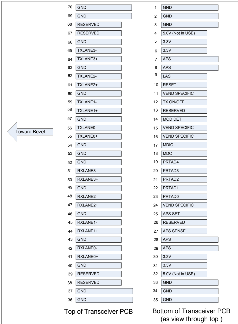
Figure 1. X2 Transponder Electrical Pad Layout
