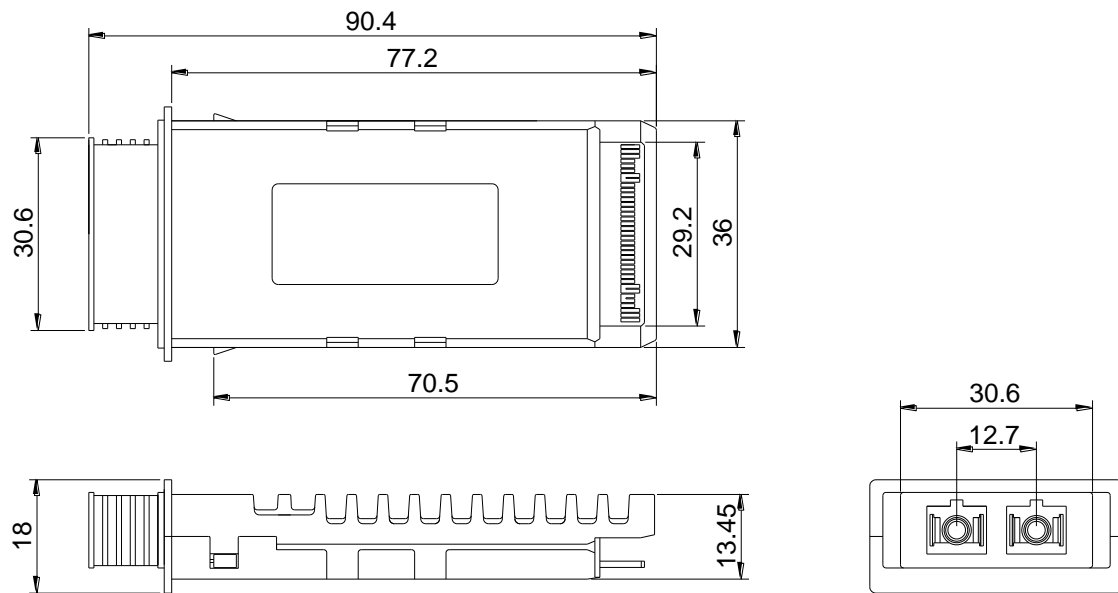
Figure 4. Outline Drawing
