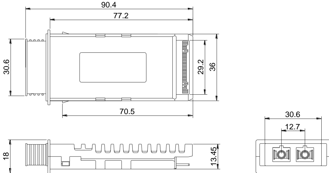
Figure 4. Outline Drawing
