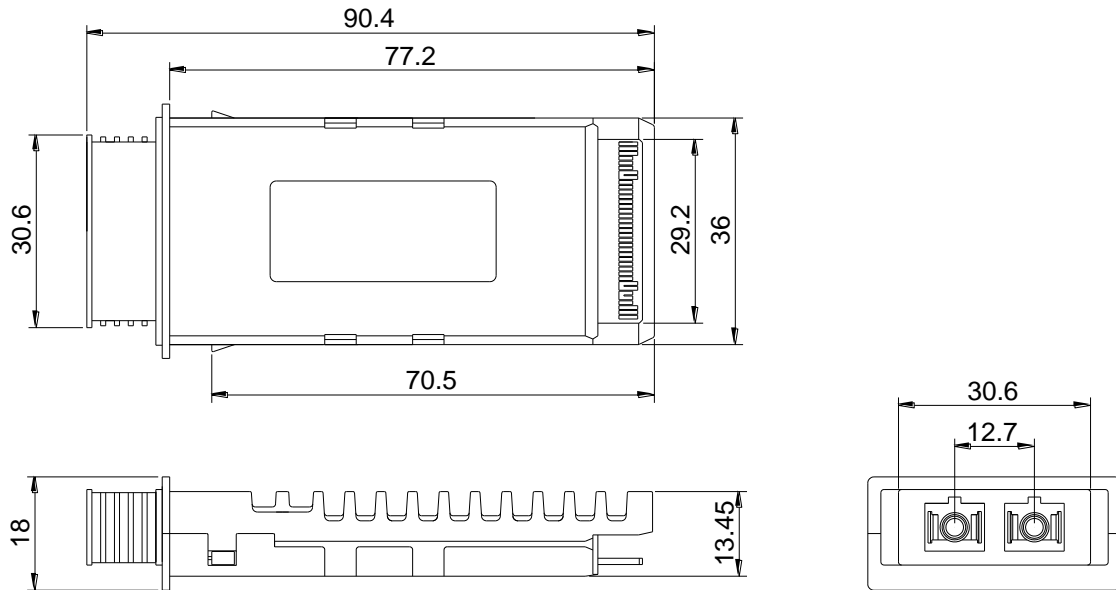
Figure 4. Outline Drawing
