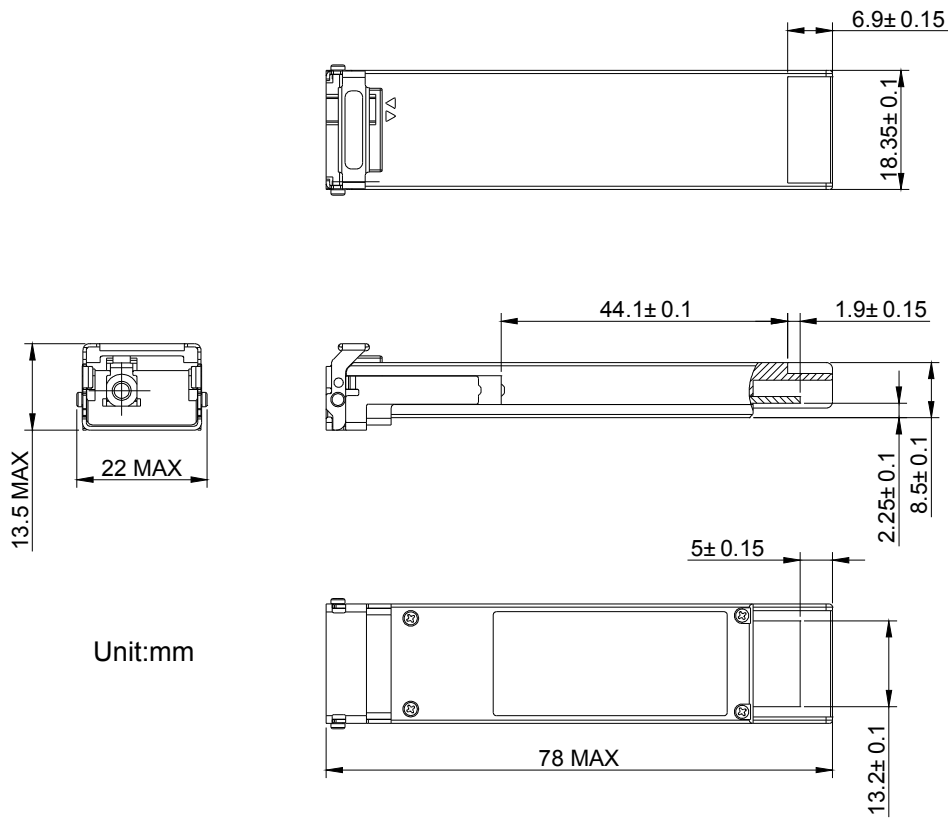
Figure 4. Outline Drawing
